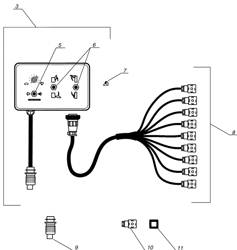
Complete No. : 1 ( Standard chute )
