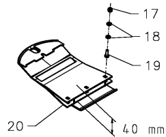
Optional Equipment 3 Set of 4 pcs.
